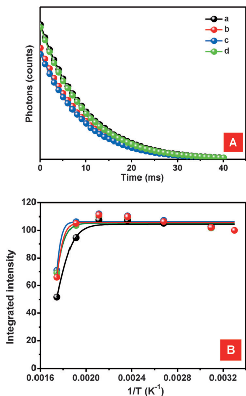
Figure 6. A) PL decay curves at 303 K and B) integrated red PL intensity as a function of temperature (303–573 K) for KSFM-MOPAl samples prepared with various OP concentrations: 0.00 M (a), 0.01 M (b), 0.05 M (c), and 0.10 M (d). The solid lines represent the result of fitting to the expression I_T/I_0 = [1 + D e^{(-E_a/kT)}]^{-1} .
